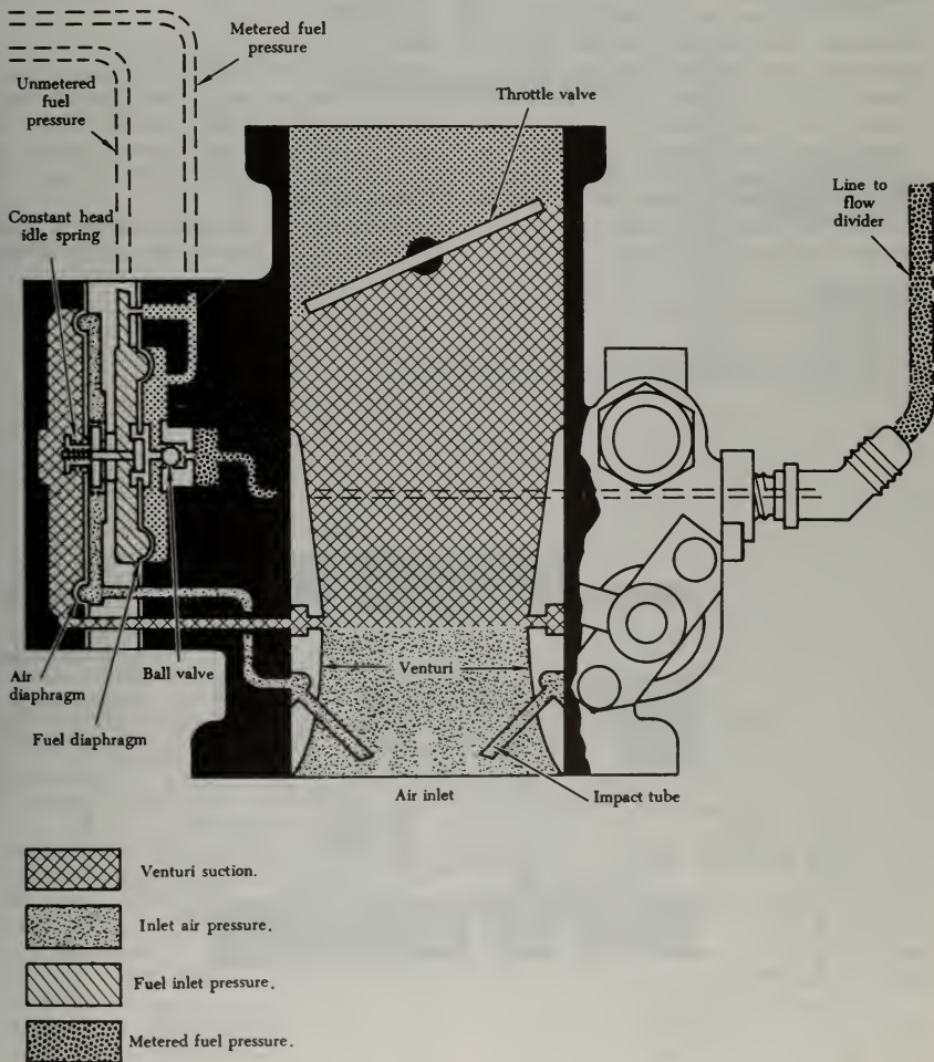
FIGURE 3-32. Airflow section of a fuel injector.
